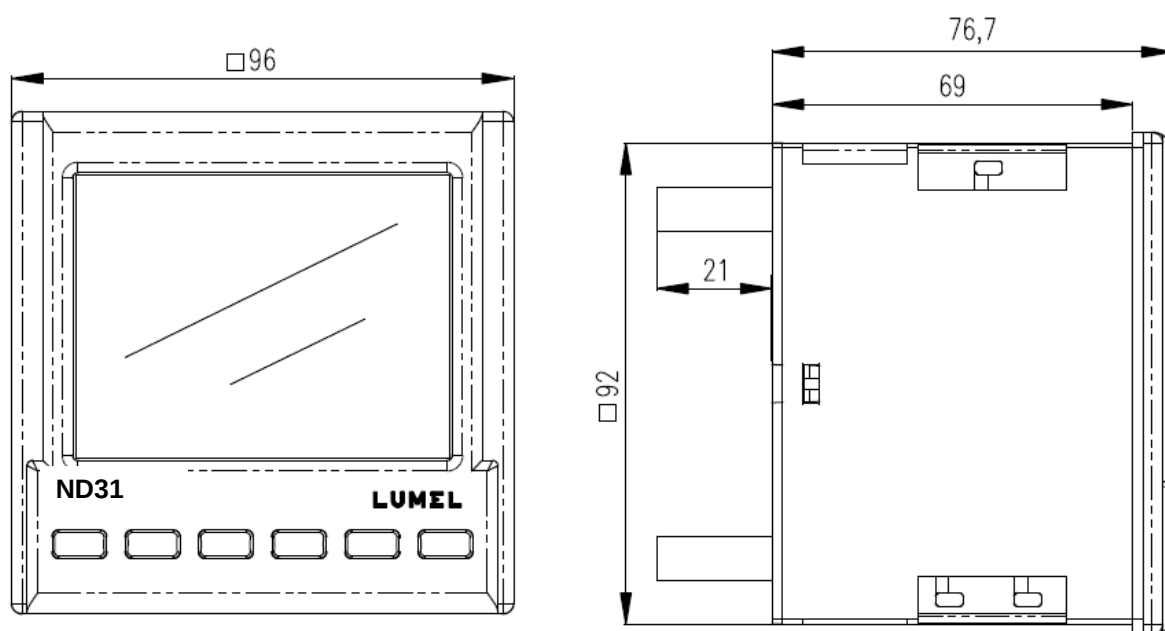
Fig. 3. Overall dimensions of the ND31 meter
