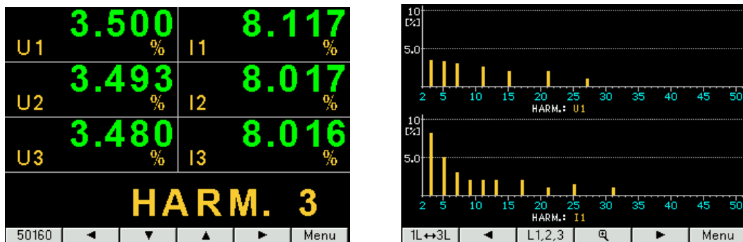
Fig. 19. Screens 11 and 12 - visualization of harmonics
