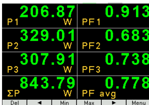
Fig. 11. Screen of meter measuring mode
