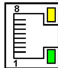
Fig. 35. View and pin numbering of the RJ45 socket
