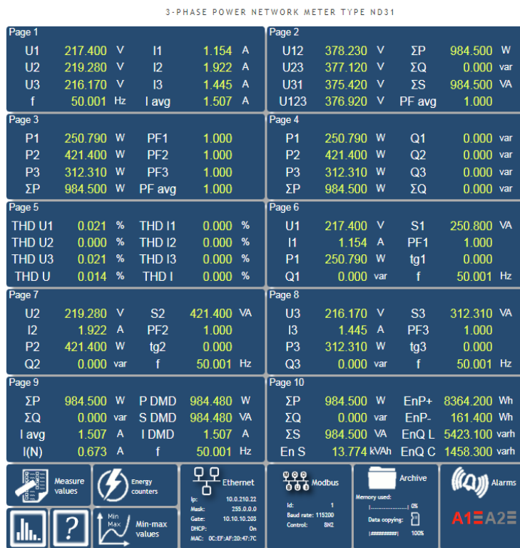
Fig. 36. View of the meter website
